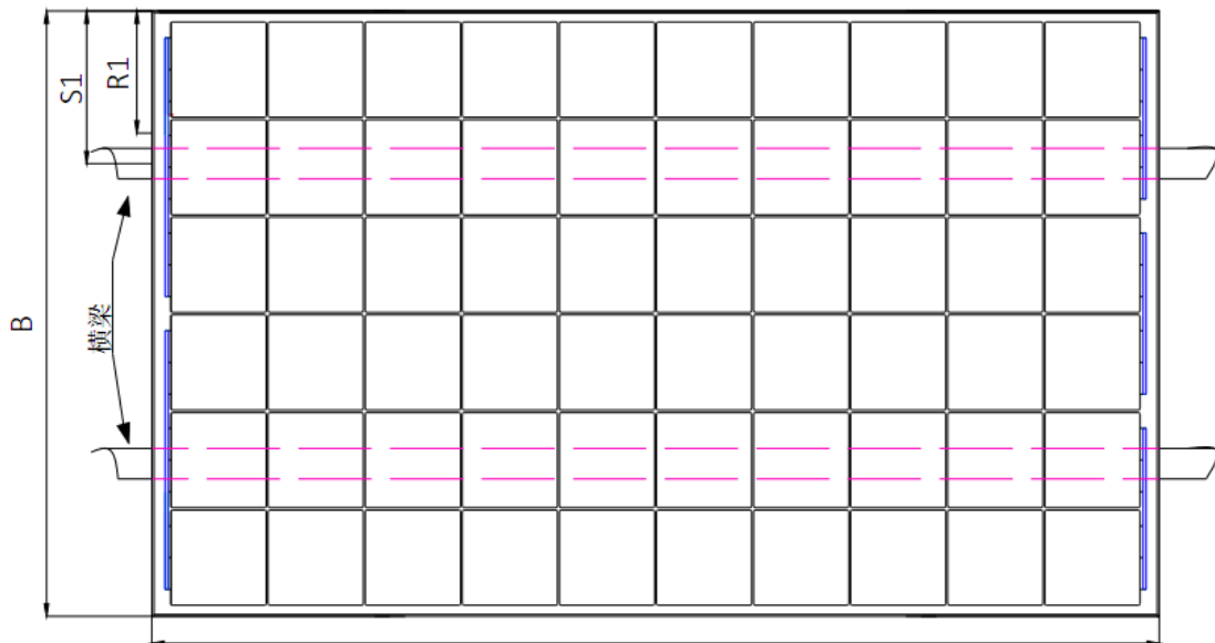
Figure 8- 3 Pressing block fixing method 1
