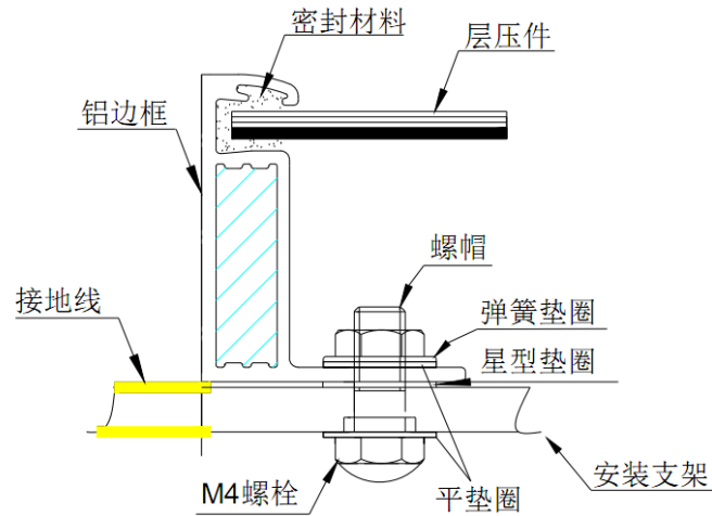
Figure 10- 1 Grounding diagram
