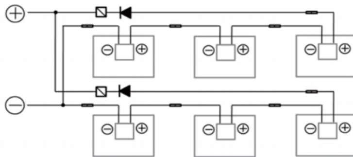
Figure 9- 3 Series-parallel connection
