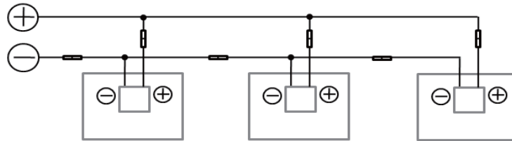
Figure 9- 2 Parallel connection
